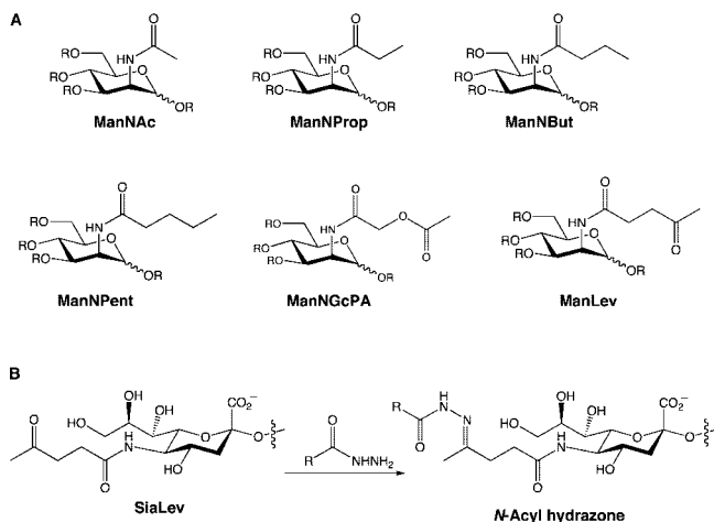
Figure 5. (A) Mannosamine derivatives used for metabolic labeling ( R = H or Ac ) and (B) chemoselective labeling reaction after treatment of cells with ManLev ( R = \text{biotin} ).
