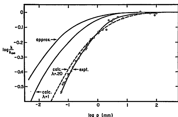
FIG. 2. Pressure dependence of the reduced-rate constant for the decomposition of cyclobutane at 722°K.
