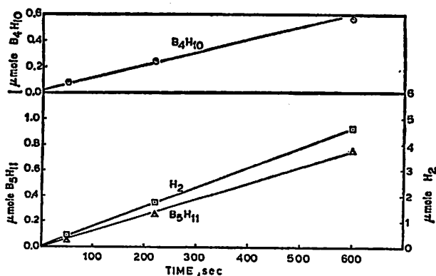
FIG. 2. Diborane photolysis. Plot of products vs irradiation time for a diborane pressure of 0.25 cm and low light intensity.
