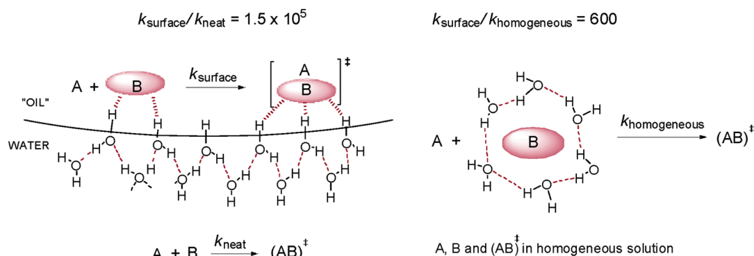
Figure 1. Summarizing cartoon of the on-water catalysis in comparison to the neat and aqueous homogeneous reactions.
