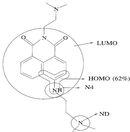
Figure 4. The various diabatic states and the relevant orbitals: |g\rangle , (\text{HOMO})^0(\text{LUMO})^0(\text{N4})^2(\text{ND})^2 ; |e\rangle , (\text{HOMO})^1(\text{LUMO})^1(\text{N4})^2(\text{ND})^2 ; |e_{\text{CT1}}\rangle , (\text{HOMO})^2(\text{LUMO})^1(\text{N4})^2(\text{ND})^1 ; |e_{\text{CT2}}\rangle , (\text{HOMO})^2(\text{LUMO})^1(\text{N4})^1(\text{ND})^2 . About 70% of the relevant orbital of |e\rangle , which is the HOMO of the system, is localized at the 4-N (40%), 3-C, 4-C, and 10-C.
