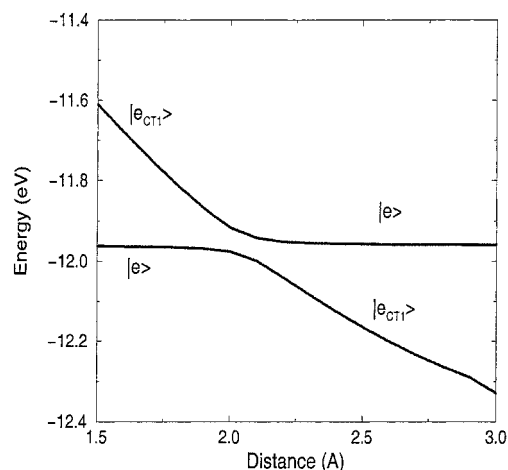
Figure 6. The calculated adiabatic curves used to obtain the electronic coupling matrix element for the electron-transfer reaction from the 9-distal N to the fluorophore.
