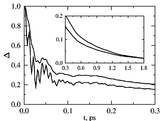
FIG. 2. The normalized correlation functions \Delta(t) [Eq. (37)] and \Delta_1(t) [Eq. (52)] are given by the upper and lower curves, respectively. The inset gives the results over a longer picosecond time interval. The spectral density of the solvent was calculated using the dielectric data of water and Eq. (61).
