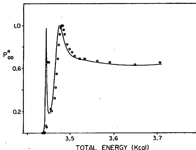
FIG. 1. Ground vibrational state transition probability for the \text{IH} + \text{I} \rightarrow \text{I} + \text{HI} reaction. The solid line is the result of Eq. (2.3) and the circles are the accurate numerical results of Ref. 4.
