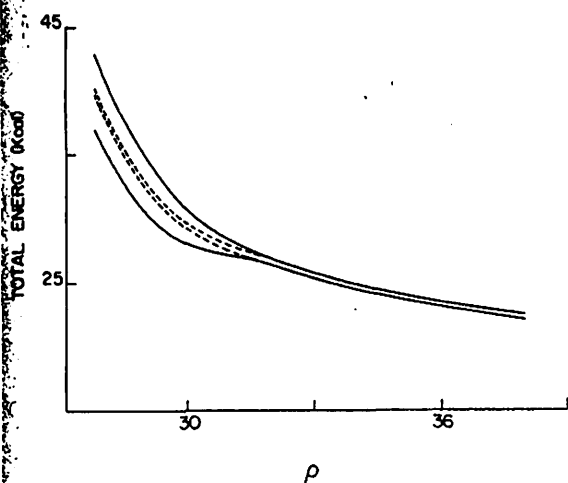
FIG. 6. Diagonal adiabatic (full line) and diabatic (dashed line) matrix elements for model surface II ( \text{ClH} + \text{Br} \rightarrow \text{Cl} + \text{HBr} ).
