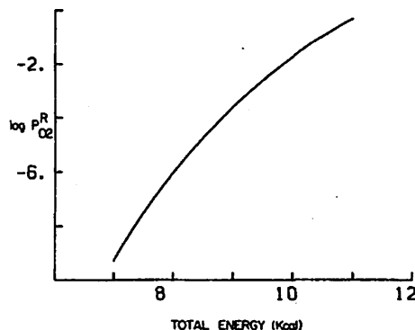
FIG. 10. The log of the transition probability for surface II ( \text{ClH} + \text{Br} \rightarrow \text{Cl} + \text{HBr} ) in the tunneling region.
