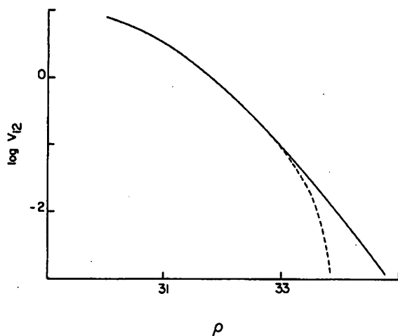
FIG. 8. The \log V_{12} vs \rho for model surface II. The dashed part of the curve corresponds to the region where Eq. (4.5) becomes unreliable (ClH+Br \rightarrow Cl+HBr).
