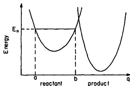
Figure 1. Model harmonic potentials for electron transfer vs. a generalized configuration coordinate q . 9
