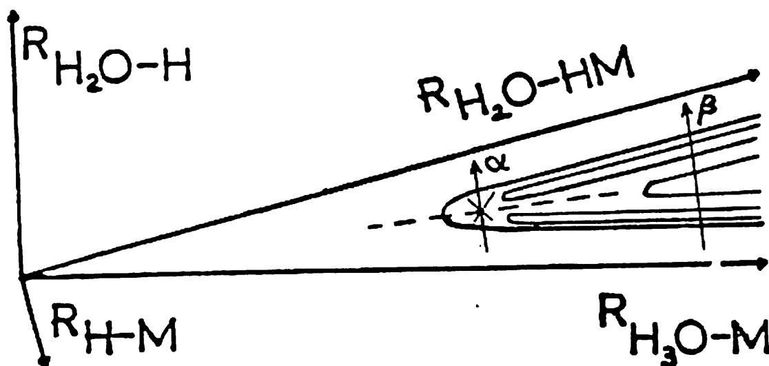
Fig. 1. Potential energy contour plot (schematic) for the three center reaction \text{H}_2\text{O}-\text{H}-\text{M} at a fixed value of the other coordinates and at a given metal-solution potential difference, for the case where the reaction is almost thermoneutral (symmetric). The rotated axes are scaled \text{H}_2\text{O}-\text{HM} and \text{H}-\text{M} distances (between O and the center of mass of HM and between H and M). 9 The configurations along the dashed line form the conventional transition state, and X denotes the saddle-point on the potential energy surface. Reaction paths \alpha and \beta are described in the text.
