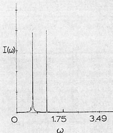
FIG. 3. Spectrum for the function x(t) + y(t) using the trajectory in Fig. 1 and computed from Eq. (2.10).
