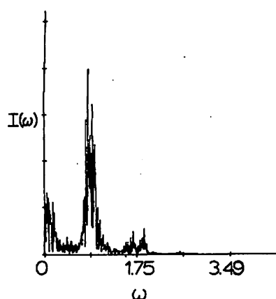
FIG. 5. Spectrum for a two-dimensional system with the Hamiltonian (3.1) and \omega_x^0 = \omega_y^0 = 1 , \lambda = 0.1118 , \eta = -1/3 , E = 11.0 .
