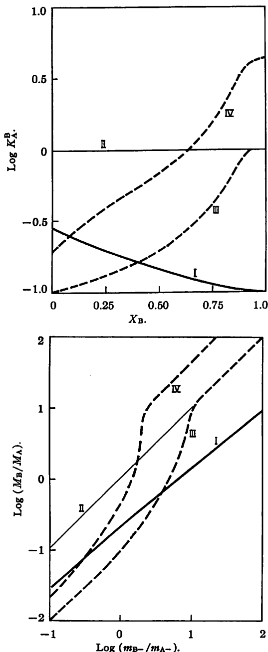
Figs. 4 and 5.—Calculated curves for selectivity of anions A and B for the following sets of postulates: I, R_A = 0.1 , B not associated; II, R_A = 0.1 , R_B = 0.1 ; III, C_A = 0.1 , B not associated; IV, C_A = 0.1 , R_B = 0.1 .
