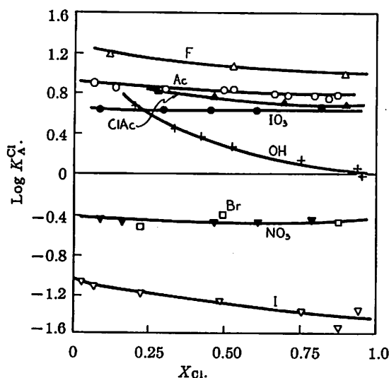
Fig. 1.—Selectivity coefficients measured against chloride with resin DVB 8 for the following anions: fluoride ( \Delta ); acetate (O); chloroacetate ( \Delta ); iodate ( \bullet ); bromide ( \square ); nitrate ( \nabla ); iodide ( \nabla ); hydroxide (+).
