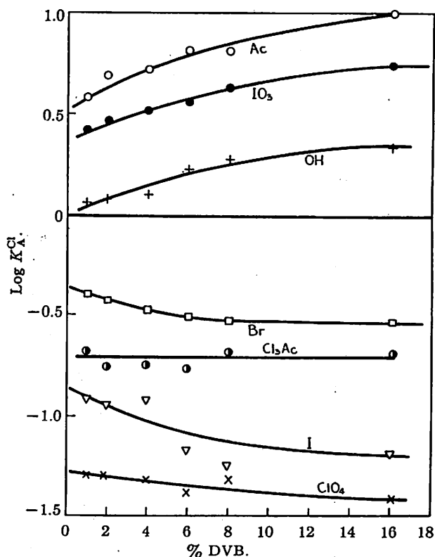
Fig. 3.—Selectivity coefficients measured against chloride for various DVB resins at X_{Cl} \approx 0.5 for the following anions: acetate (O); iodate ( \bullet ); hydroxide (+); bromide ( \square ); trichloroacetate ( \bullet ); iodide ( \nabla ); perchlorate ( \times ).
