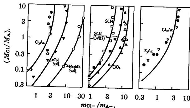
Fig. 6.—Experimental points and curves calculated based upon the postulate of random-clustered systems for anion-exchange processes with resin DVB 8 and chloride with the following anions: trichloroacetate (○); p -toluenesulfonate (▼); \beta -naphthalenesulfonate (○); thiocyanate (□), with DVB 2 (■); perchlorate (Δ), with DVB 2 (▲); dichloroacetate (▽); trifluoroacetate (●).
