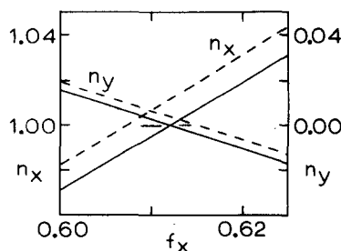
FIG. 4. Enlarged drawing of Fig. 3. The dashed line shows n_x and n_y for E=1.7000 which is the energy level for the uncoupled system having \lambda=0 , cf., Eq. (1). The shift in the n_x=1 , n_y=0 energy level due to the coupling for the nonzero \lambda is clearly seen.
