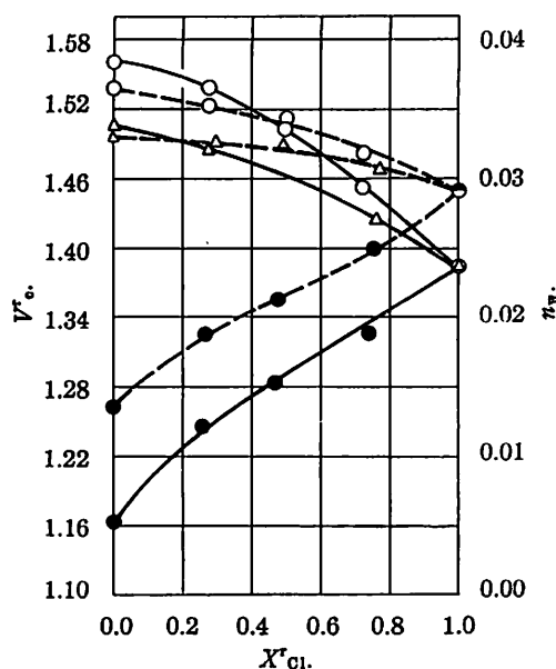
Fig. 2.—Specific volume V_r^0 (solid lines) and specific water content in moles n_w^* (dotted lines) for DVB 8 resin in various mixed anionic states: chloride-acetate (O); chloride-iodate ( \Delta ); and chloride-perchlorate ( \bullet ).
