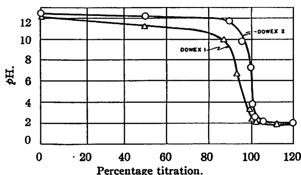
Fig. 1.—Titration of Dowex 2 (O) and Dowex 1 (Δ) resins (DVB 8) in 1 m potassium chloride, under equilibrium conditions.
