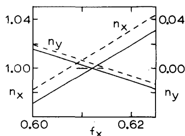
FIG. 4. Enlarged drawing of Fig. 3. The dashed line shows n_x and n_y for E=1.7000 which is the energy level for the uncoupled system having \lambda=0 , cf., Eq. (1). The shift in the n_x = 1 , n_y = 0 energy level due to the coupling for the nonzero \lambda is clearly seen.
