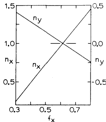
FIG. 3. The quantum numbers n_x and n_y computed from various trajectories. All of the trajectories have the same total energy E=1.6870 and differ in f_x , the energy initially in the x oscillator. This total energy is clearly a semiclassically allowed energy level of the system since both n_x and n_y are integers at f_x=0.6120 . The system has the Hamiltonian of Eq. (1) with frequencies such that \omega_x^2=0.49 , \omega_y^2=1.69 and coupling parameters \lambda=-0.1 , \eta=0.1 .
