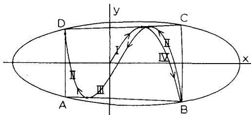
FIG. 2. A portion of the trajectory of Fig. 1 with the four branches of the momentum functions P_x(xy) , P_y(xy) generated by it marked. The dots indicate the points where the trajectory touches the caustic curves, which are the nearly straight lines forming the sides of the "box" ABCD .
